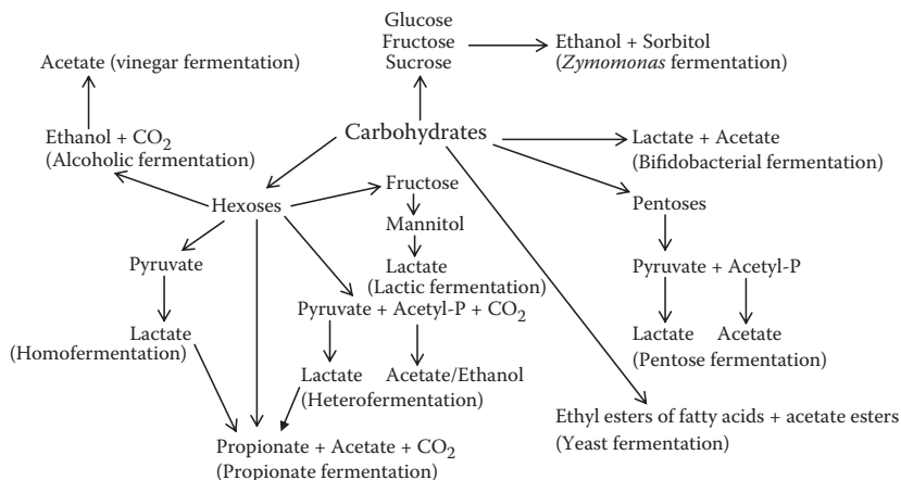
FIGURE 2.1 A simplified scheme of flavor compound formation from carbohydrates via microbial fermentation.
