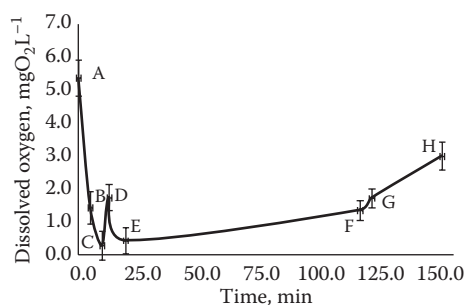
FIGURE 12.4 Dissolved oxygen during apple juice processing. (A) Pressing; (B) 5 minutes after pressing; (C) 10 minutes after pressing; (D) pectinase addition; (E) heating at 40°C for enzyme action; (F) end of depectinization process; (G) racking; (H) filtration. Brazilian cider processing conditions: commercially discarded apples (Gala and Fuji), temperature at 25°C, 975 m a.s.l., and pilot plant of the apple work group.
