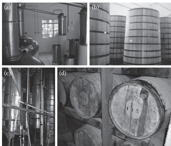
FIGURE 38.1 (a) Copper alembics for distillation of traditional cachaca, (b) umburana barrels to store cachaca, (c) stainless steel columns for industrial cachaca production, and (d) oak barrels for cachaca aging.
