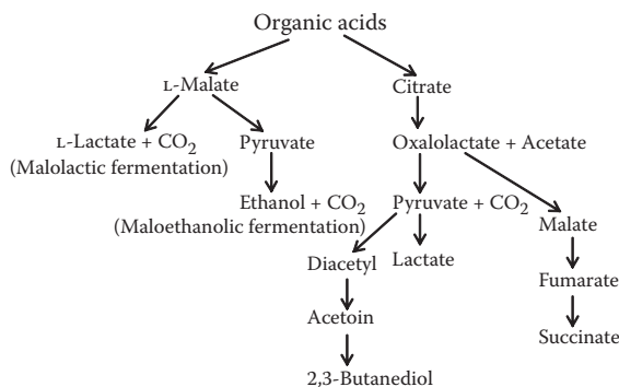
FIGURE 2.5 A simplified scheme of flavor compound formation from organic acids via microbial fermentation.
