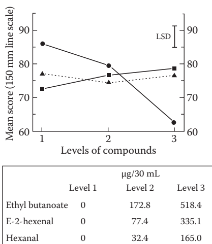
FIGURE 9.2 Mean intensities for overall liking of kiwifruit model solution with various levels of added compounds. Square, ethyl butanoate; circle, E-2-hexenal; triangle, hexanal. Solid lines represent significant effects. (From Gilbert, J. M., et al.: J Sens Stud. 1996, 11(3), 247–259. Copyright Wiley-VCH Verlag GmbH & Co. KGaA. Reproduced with permission.)
