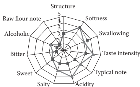
FIGURE 29.5 Results of sensory evaluation on the bread made with Lb1 liquid sourdough (▲) and on the bread made with bakers' yeast (■). (Reprinted from Food Microbiology , 24, Carnevali P. et al., Liquid sourdough: Industrial Application Perspectives, pp. 2–4, Copyright (2007), with permission from Elsevier.)
