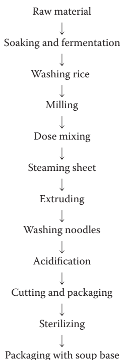
FIGURE 30.1 Flowchart of fermented rice noodle processing.
