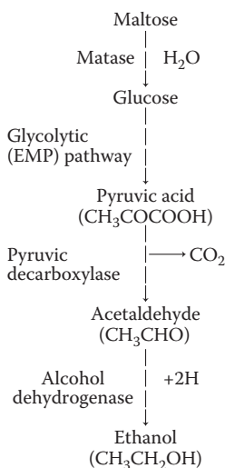
FIGURE 33.2 Fermentation of maltose to ethanol and carbon dioxide.
