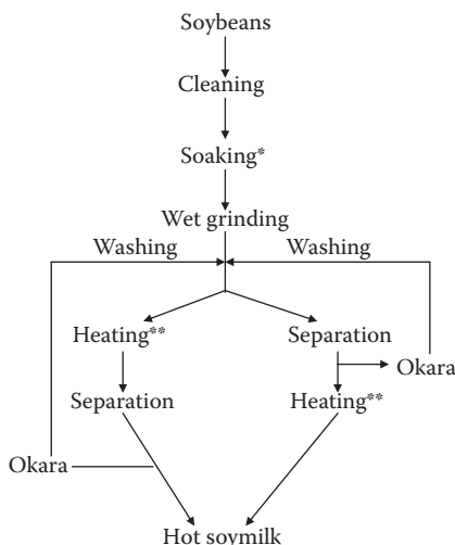
FIGURE 8.1 Preparation of soymilk for tofu making. *15°C to 20°C for 8 to 10 hours or 10°C to 15°C for 12 to 16 hours. **98 to 105°C for 2 to 5 minutes.
